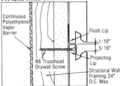
TYPICAL WALL CROSS SECTION
