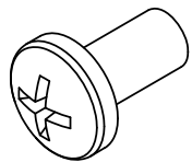
4X.PAN CROSS HEAD HALF THREAD SCREW 5/16"- 18X0.875"
