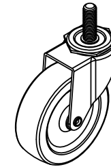
4X. 4"CASTER W/1/2"-13X1.5"THREAD
